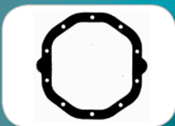
DG10C - Holden Commodore VC-VK
